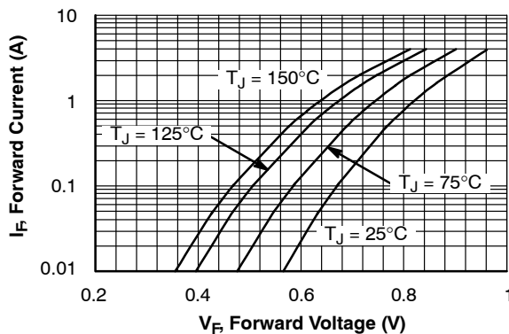
Figure 4. Typical Forward Characteristics
