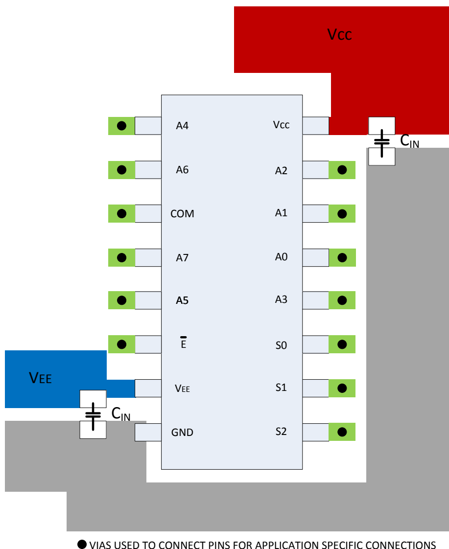
Figure 14. Layout Example
