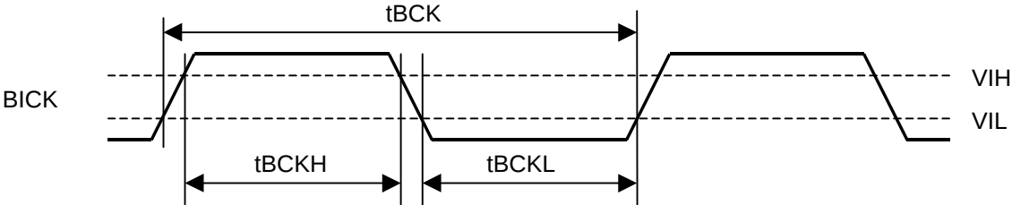
Clock Timing
