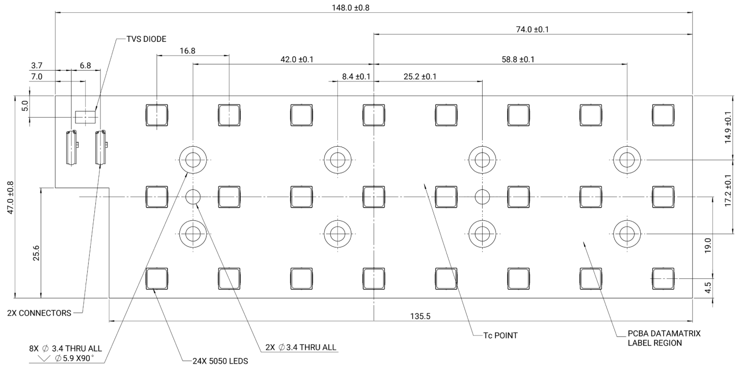
Top View
