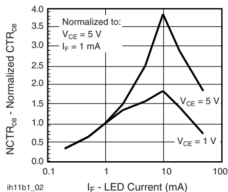
Fig. 2 - Normalized Non-Saturated and Saturated \text{CTR}_{\text{CE}} vs. LED Current
