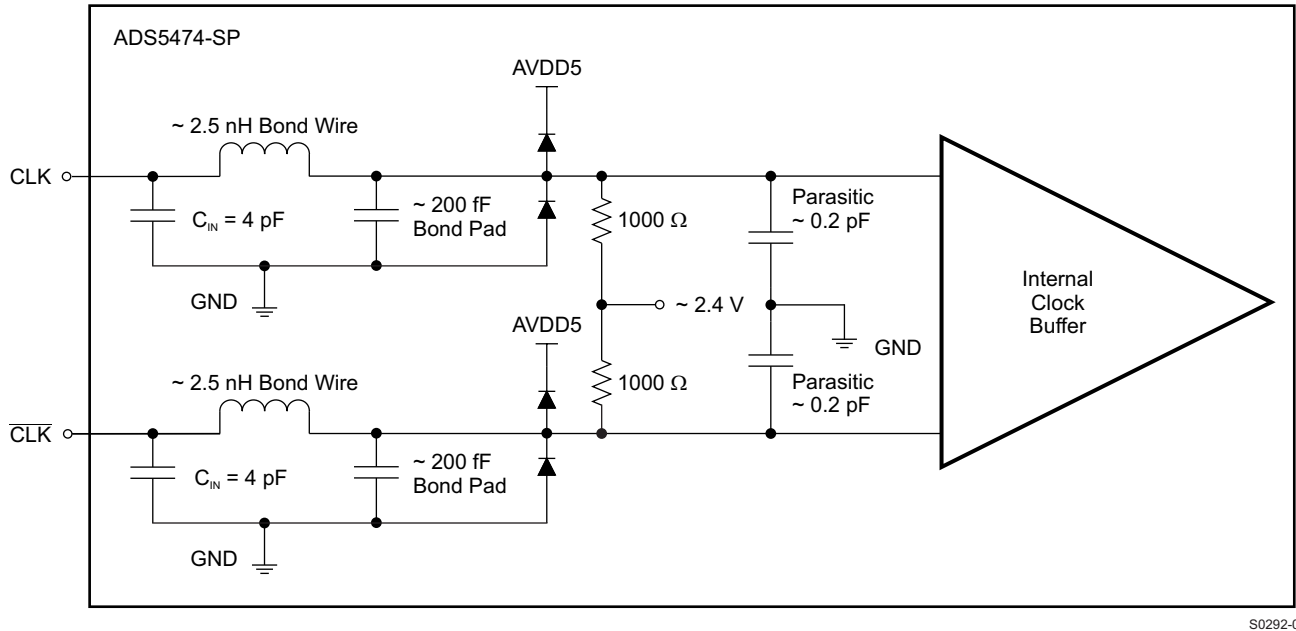
Figure 34. Clock Input Circuit
