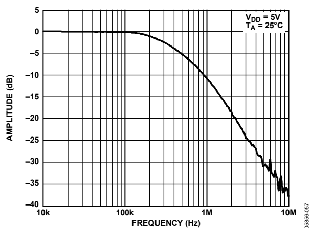
Figure 50. Multiplying Bandwidth
