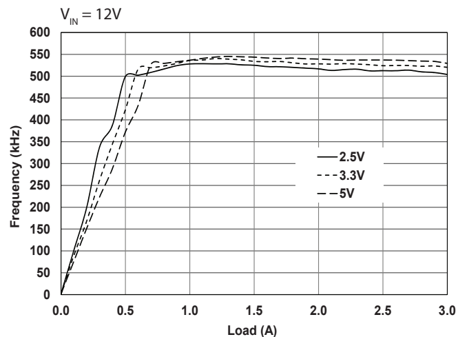
Switching Frequency vs Load - 2.5V, 3.3V, 5V
