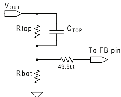
Figure 2 — Output Voltage Selection
