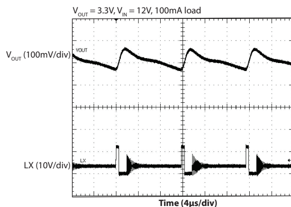
Power Save Switching - 100mA Load
