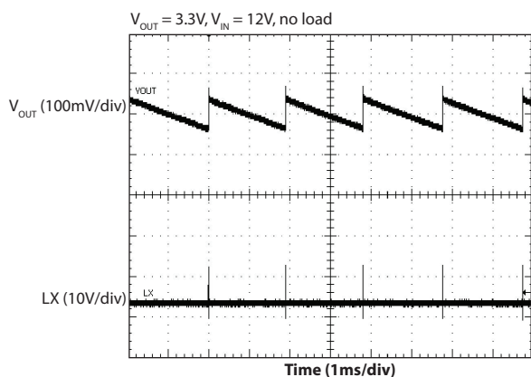
Power Save Switching - No Load
