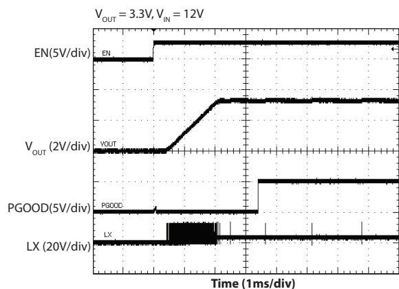
Startup - EN controlled
