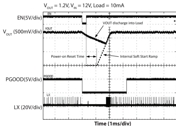
Pre-bias Startup
