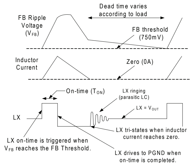
Figure 4 — Power-save Operation
