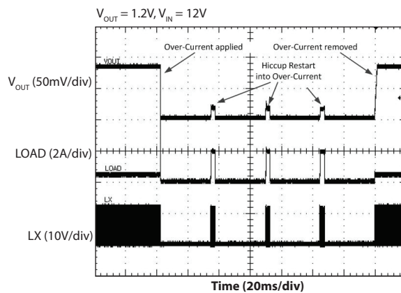
Hiccup Recovery from Over-Current
