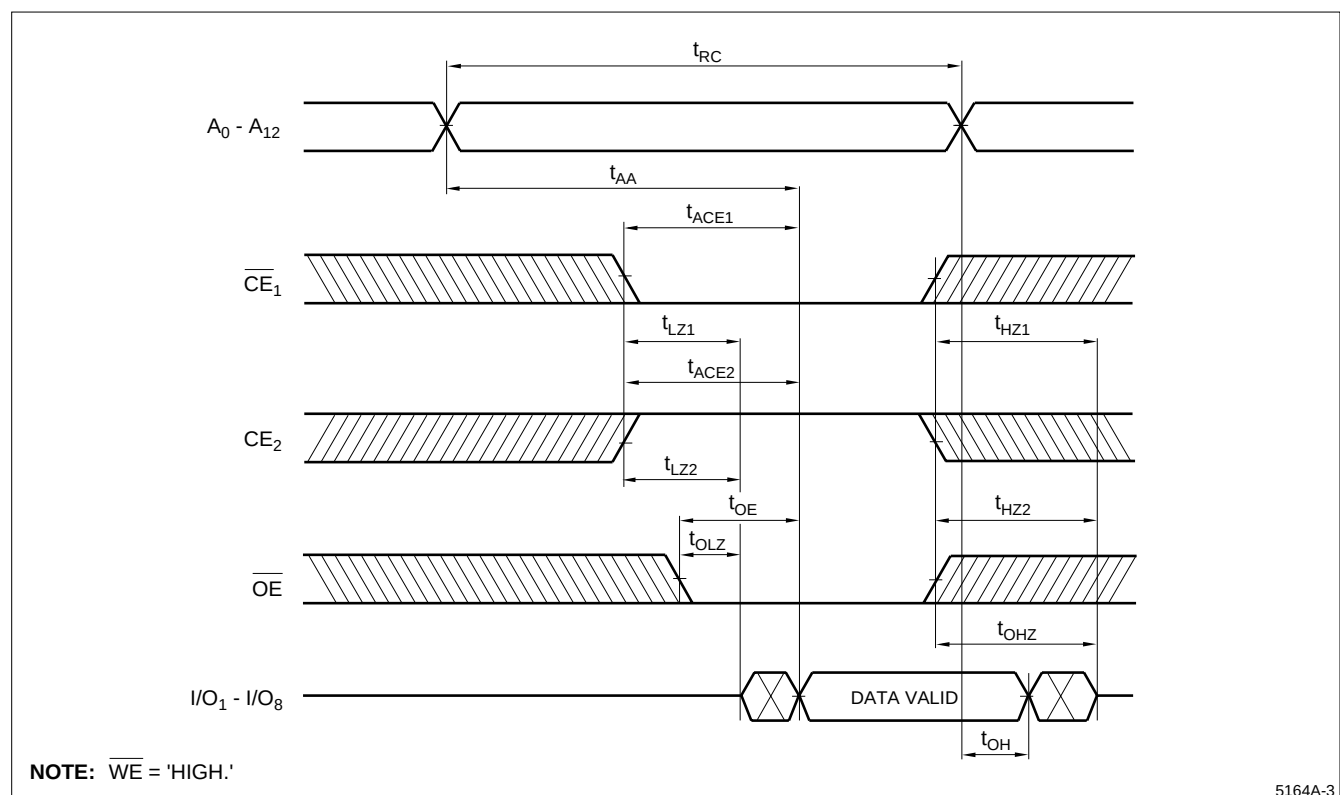
Figure 5. Read Cycle
