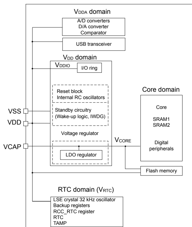
Figure 2. STM32C53xxx power supply overview
