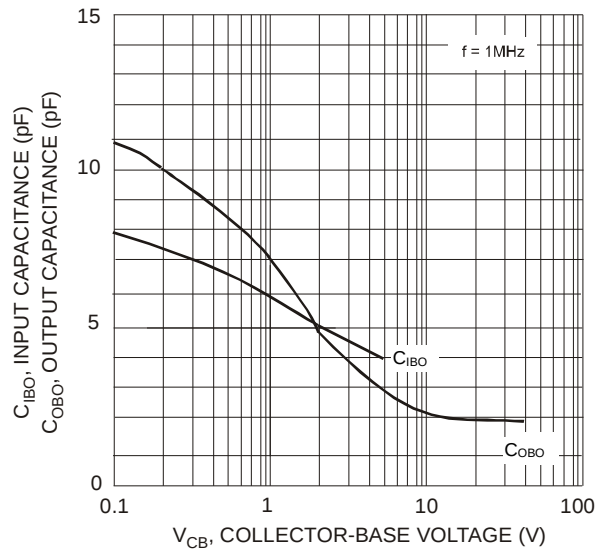
Fig. 5, Input and Output Capacitance vs. Collector-Base Voltage
