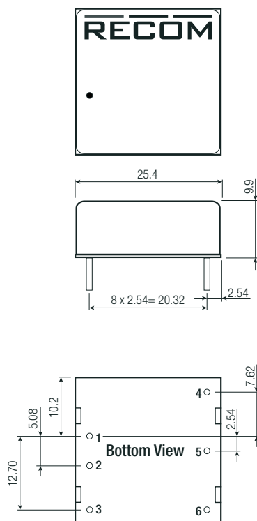
Dimension Drawing (mm)
