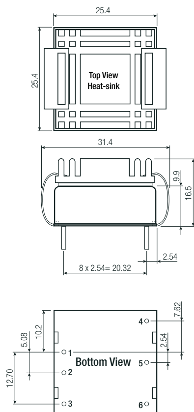
Dimension Drawing with Heat-sink (mm)
