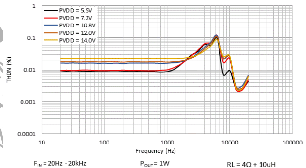
Figure 10. THD+N vs. Frequency
