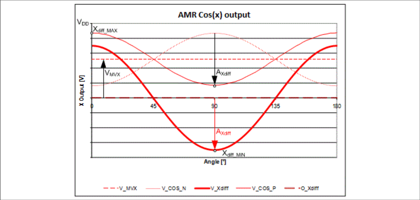
Figure 19 AMR differential output of ideal cosine
