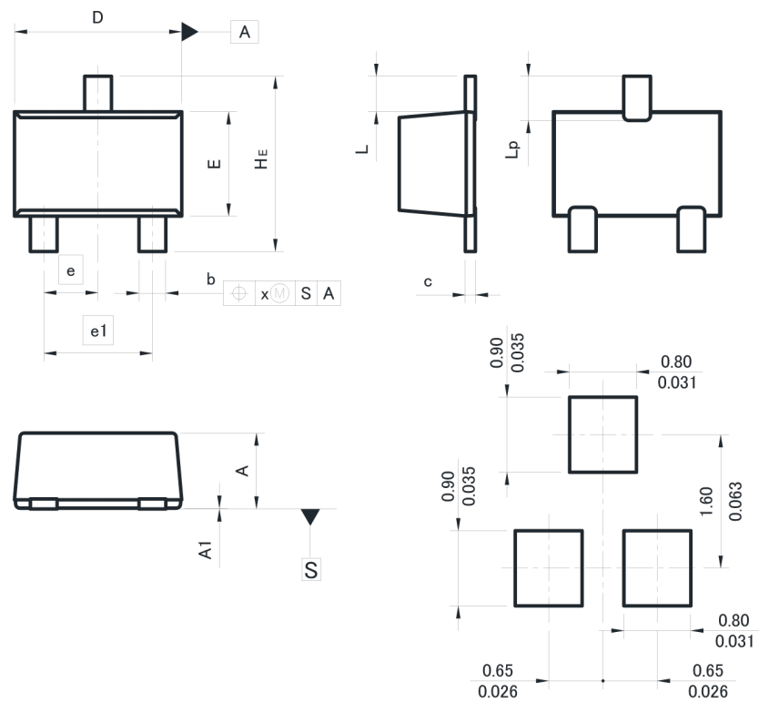
Soldering footprint
