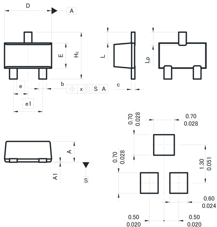
Soldering footprint Unit: ( \frac{\text{mm}}{\text{inches}} )
