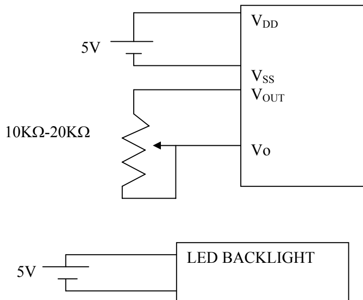
Power Supply
