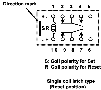
Single coil latch type
