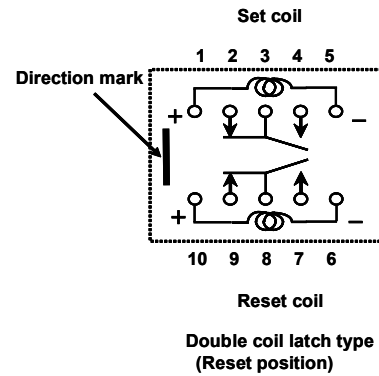
Double coil latch type
