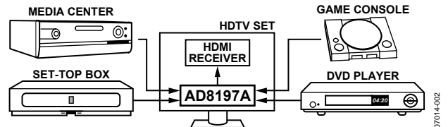
Figure 2. Typical HDTV Application
