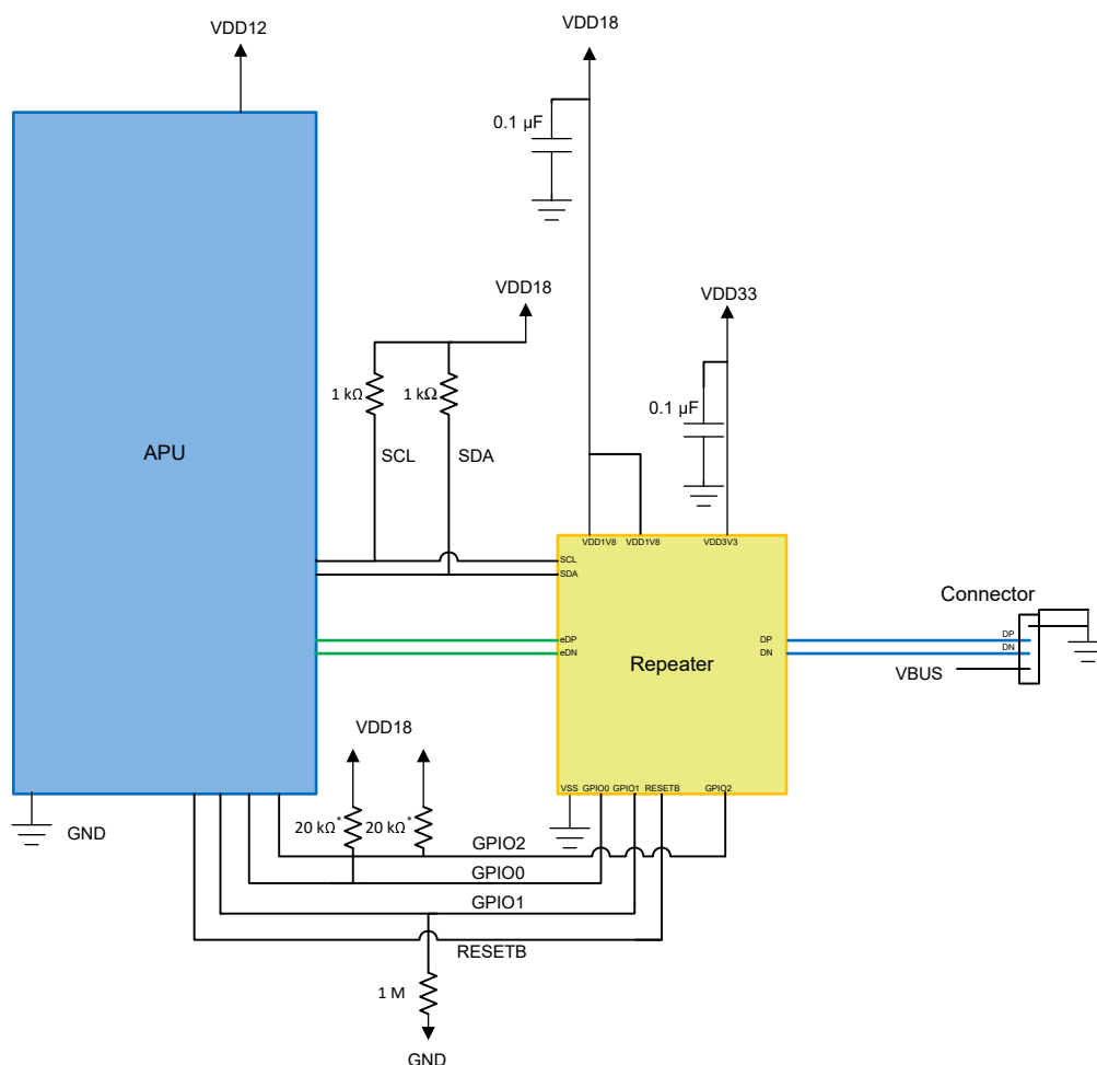
Figure 11-1. Typical System Implementation Using 1.8V I²C Variant
