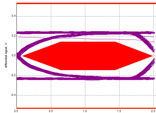
Figure 11-4. eUSB2 TX Eye Diagram with eTP1 (Terminated) Mask
