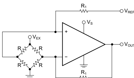
Figure 6. Bridge Amplifier Using a Single Operational Amplifier
