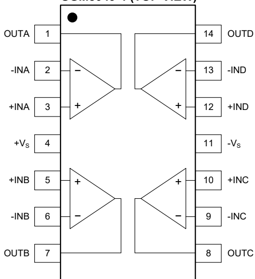
SGM8049-4 (TOP VIEW)
