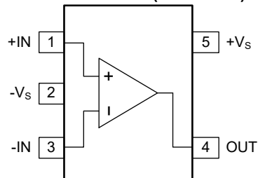
SGM8049-1BXC5G (TOP VIEW)
