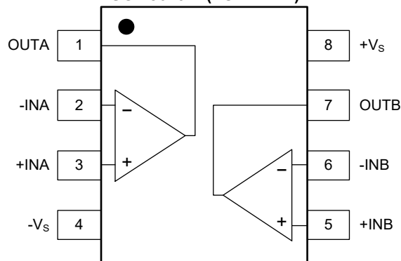
SGM8049-2 (TOP VIEW)
