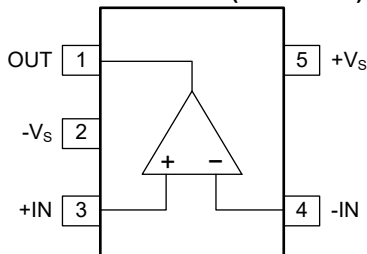
SGM8049-1XN5G SGM8049-1AXC5G (TOP VIEW)
