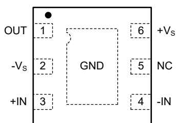
SGM8049-1 (TOP VIEW)
