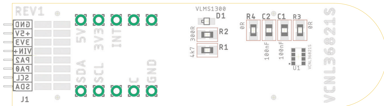
Assembly top
