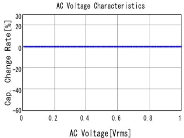
■ ECASD60J227M010K00 C-AC Voltage capchange, DC0V, 25.0
