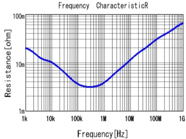
■ ECASD60J227M010K00 R DC0V, 25degC
