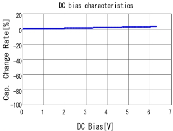
■ ECASD60J227M010K00 C-DC bias capchange, 25.0degC, AC1
