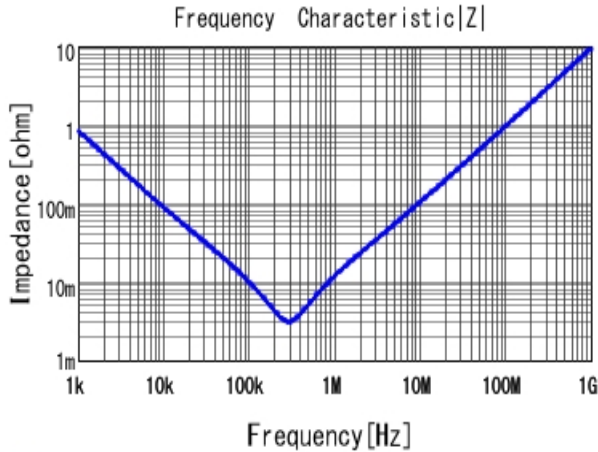
■ ECASD60J227M010K00 |Z| DC0V, 25degC
