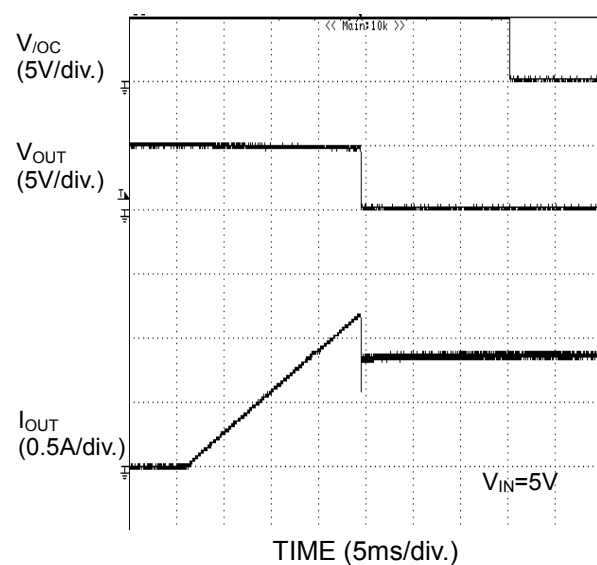
Figure 35. Over-Current Response Ramped Load
