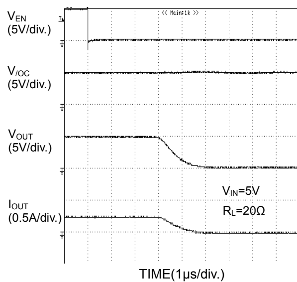
Figure 33. Output Fall Characteristic
