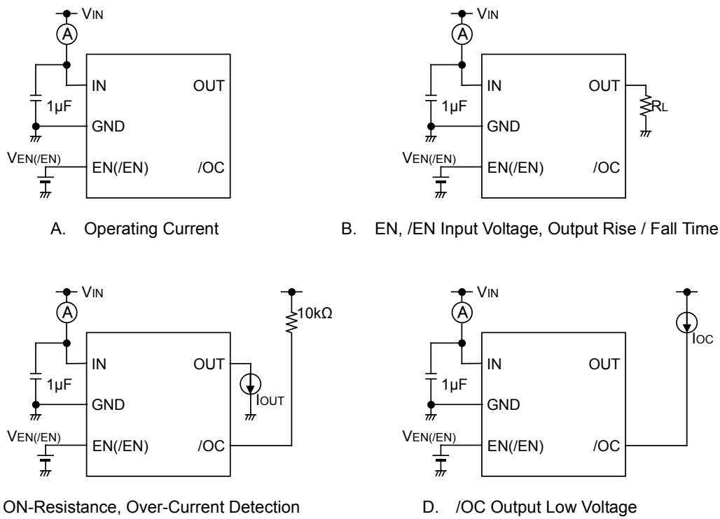
Figure 1. Measurement Circuit
