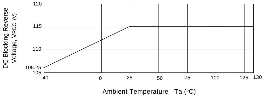
V_{R(DC)} - T_a Characteristic
