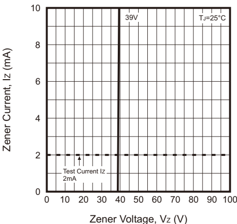
Fig.4 - Typical Zener Breakdown Capacitance
