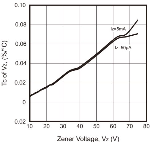
Fig.6 - Typical Temperature Coefficient of Zener Voltage
