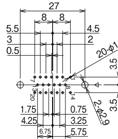
SD-1620A(09)
