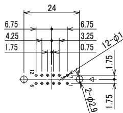
PD-1612BA(09)
