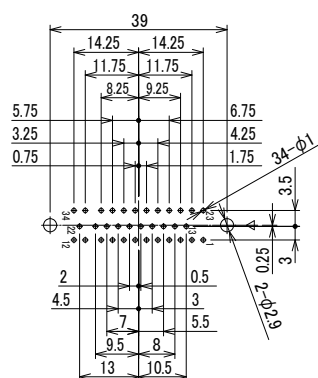
PD-1634BA(09)
