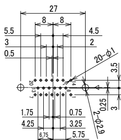
PD-1620BA(09)
