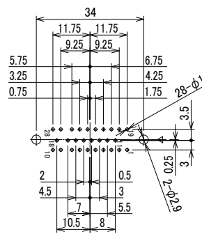
PD-1628BA(09)
