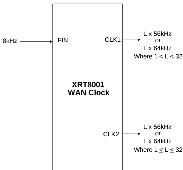
Figure 12. Illustration of the XRT8001 WAN Clock Operating in the “Forward/Slave” Mode
