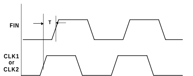
Figure 20: Timing Relationship between the FIN and the “CLK1/CLK2” outputs in Slave Mode
