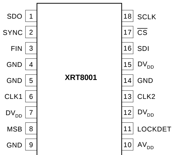
Figure 3. XRT8001 PIN OUT
