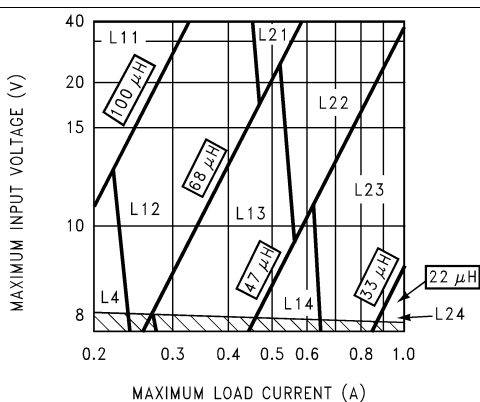
Figure 23. LM2672, 3.3-V Output
