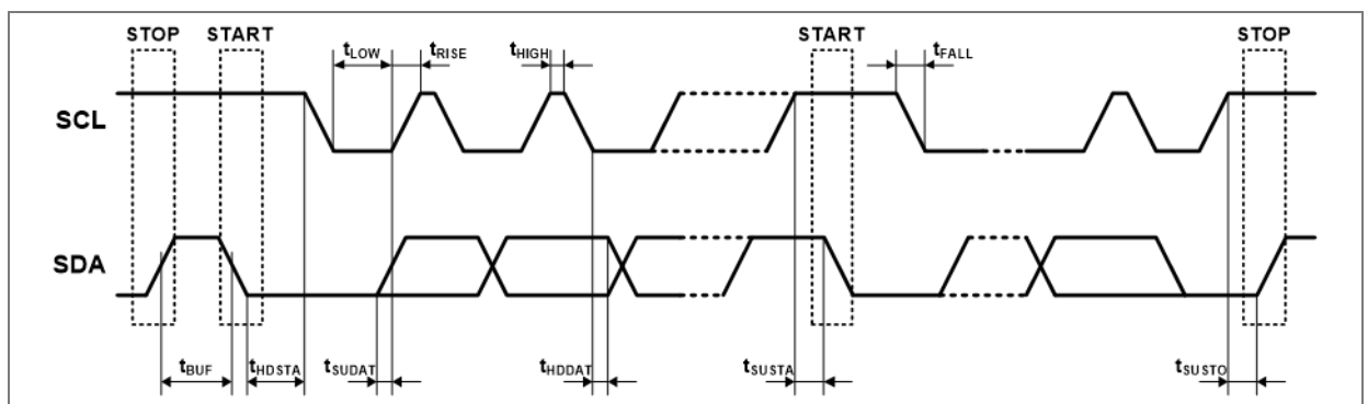
Figure 8: Serial interface timing diagram
