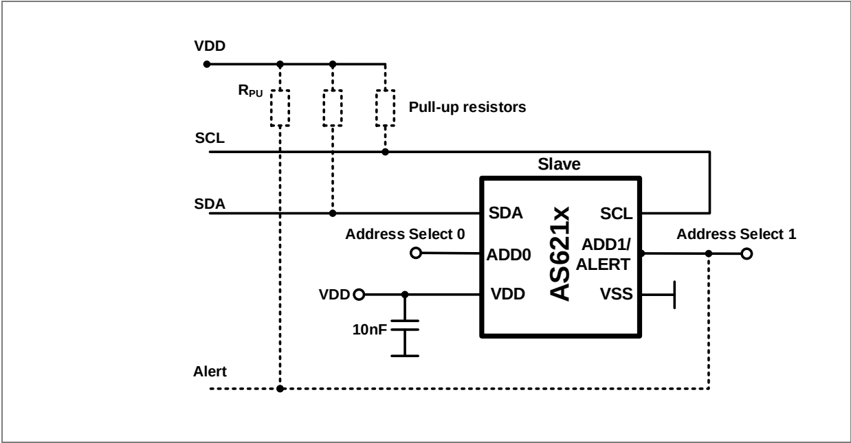
Figure 12: Schematic with external components
