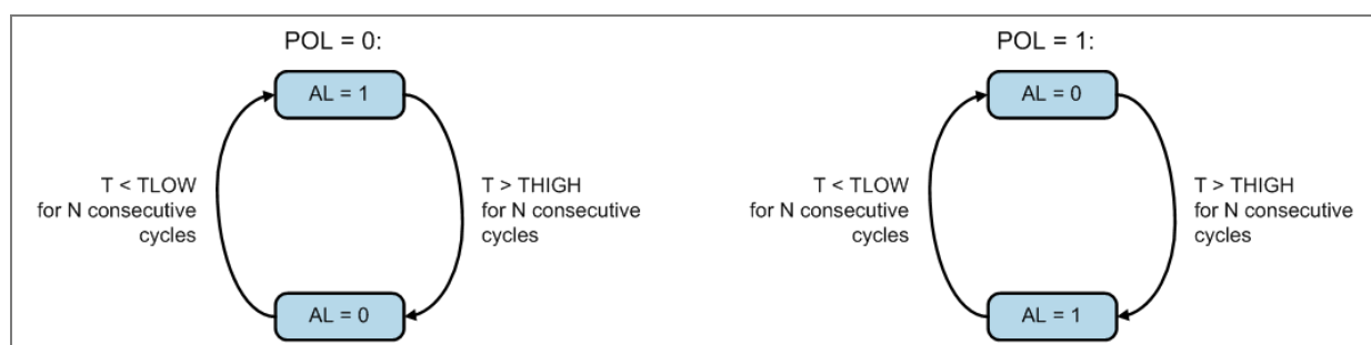
Figure 4: State diagram of the alert bit
