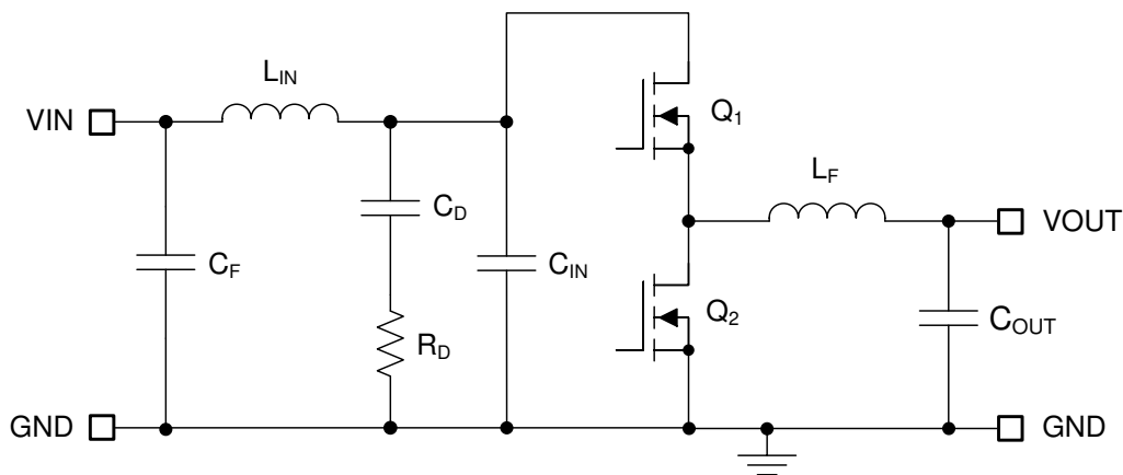
Figure 9-4. Buck Regulator With \pi -Stage EMI Filter
