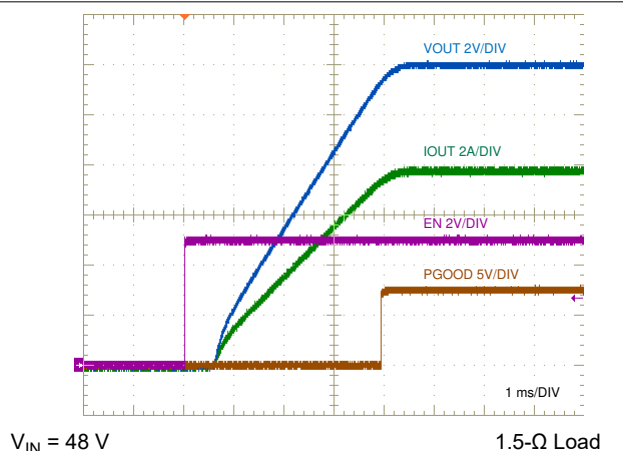
Figure 9-21. ENABLE ON, 10-A Resistive Load
