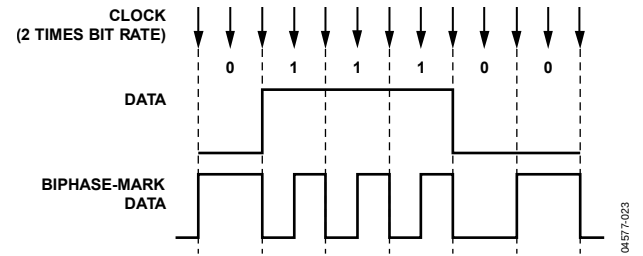
Figure 43. Biphase-Mark Encoding
