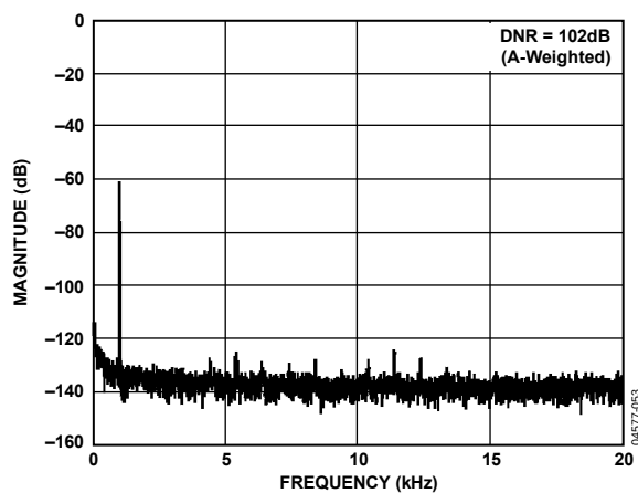
Figure 19. ADC Dynamic Range, f_s = 48 kHz
