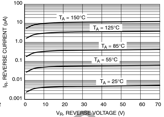
Figure 13. Leakage Current
