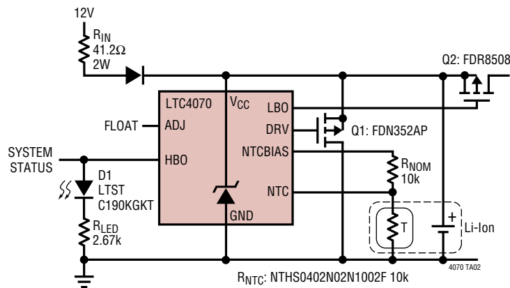
Figure 9. 12V Wall Adapter Charging with 205mA with Automatic Load Disconnect on Low Battery
