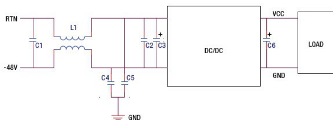
Figure 8. Conducted Emissions Test Circuit
