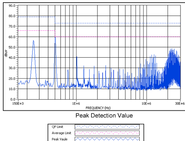
Graph 5. Conducted emissions performance, Positive Line, CISPR 22, Class A , 24Vin, full load
