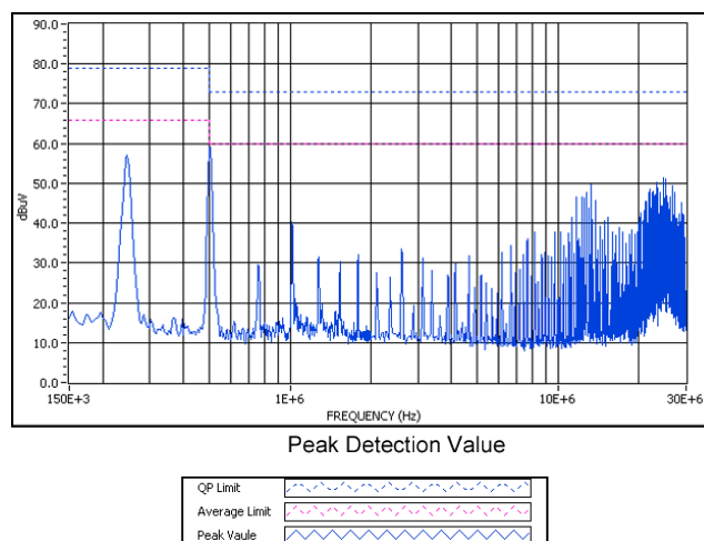
Graph 6. Conducted emissions performance, Negative Line, CISPR 22, Class A , 24Vin, full load
