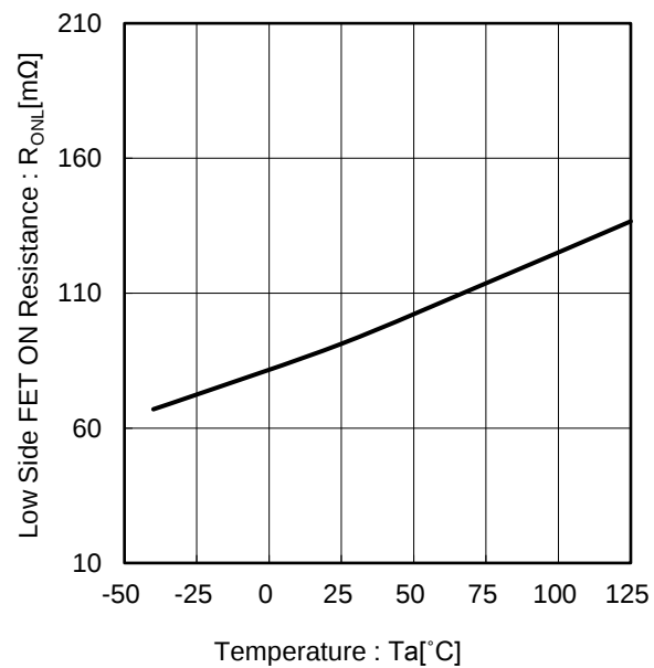
Figure 16. Low Side FET ON Resistance vs Temperature
