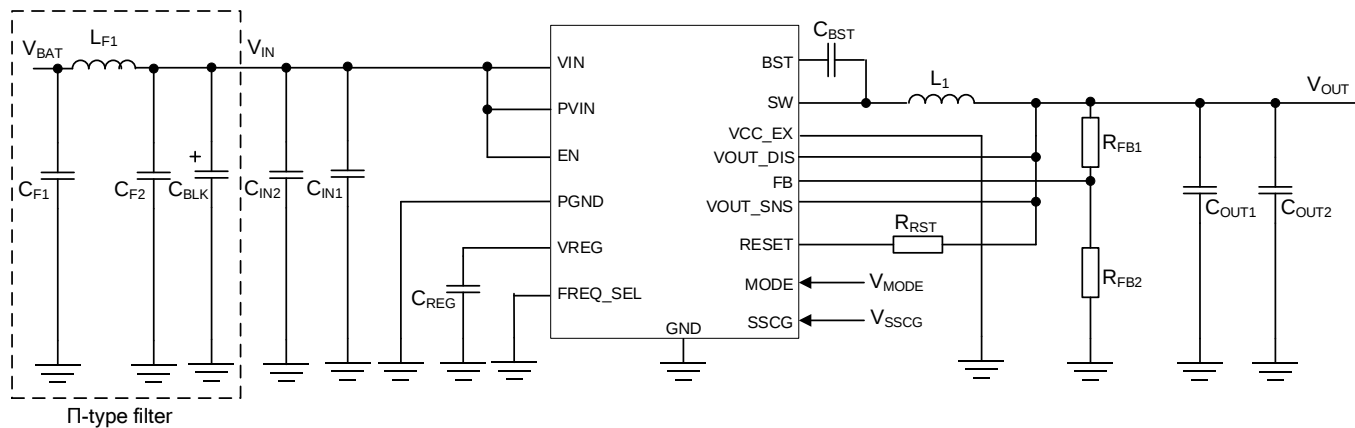
Figure 41. Reference Circuit 1
