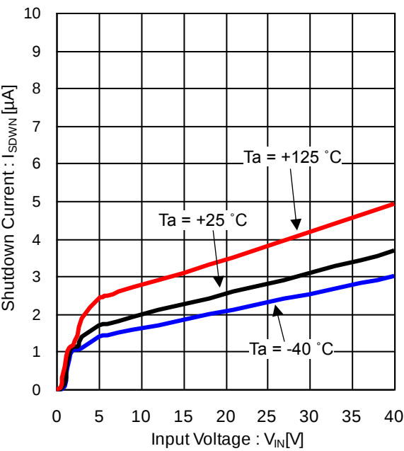
Figure 5. Shutdown Current vs Input Voltage
