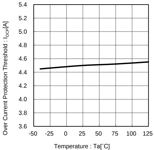
Figure 20. Over Current Protection Threshold vs Temperature
