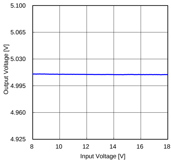
Figure 78. Line Regulation (I OUT = 3 A)
