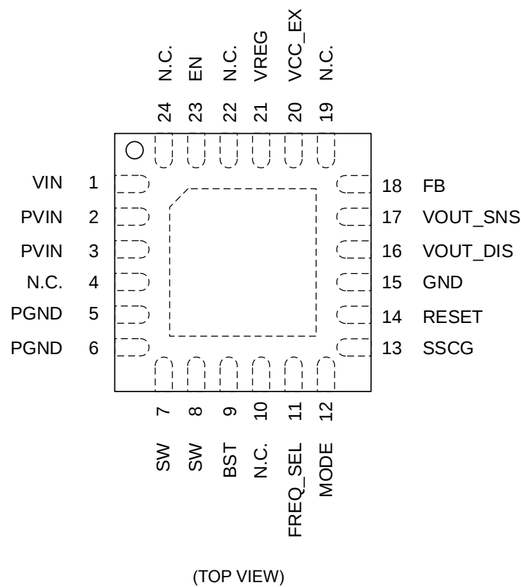
Figure 3. Pin Configuration
