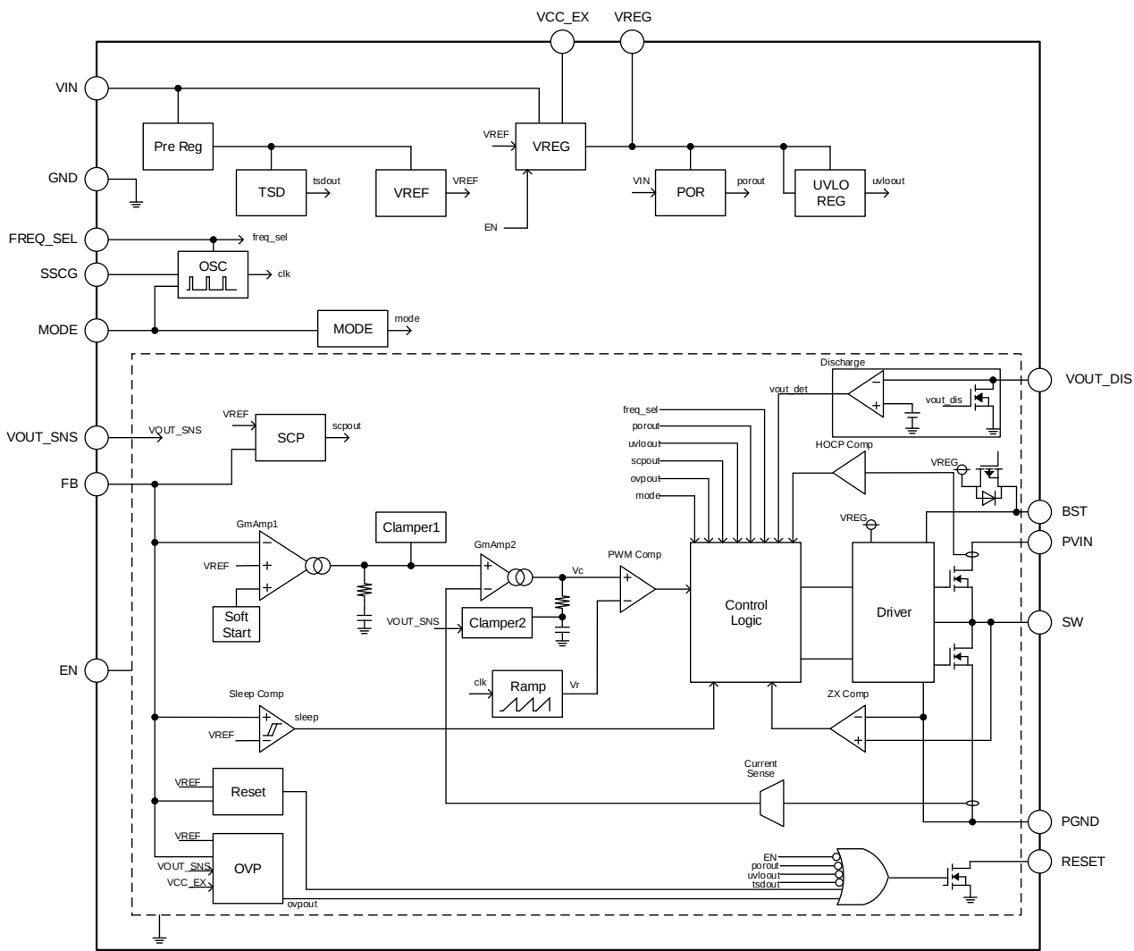
Figure 4. Block Diagram
