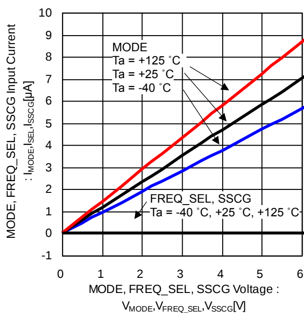
Figure 12. MODE, FREQ_SEL, SSCG Input Current vs MODE, FREQ_SEL, SSCG Voltage
