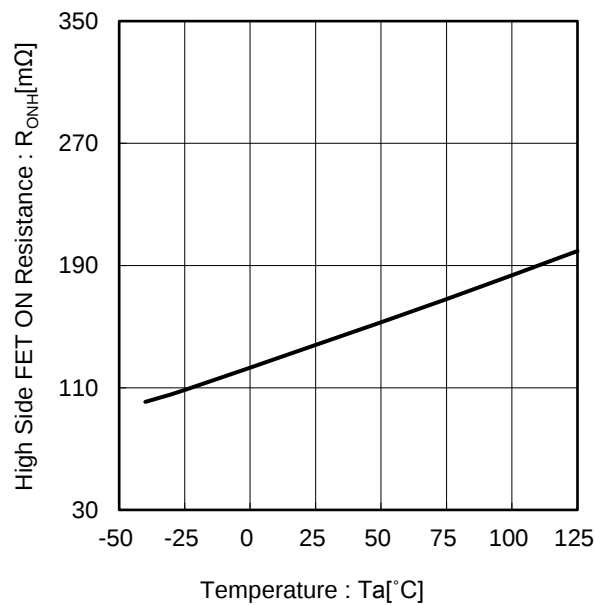
Figure 15. High Side FET ON Resistance vs Temperature
