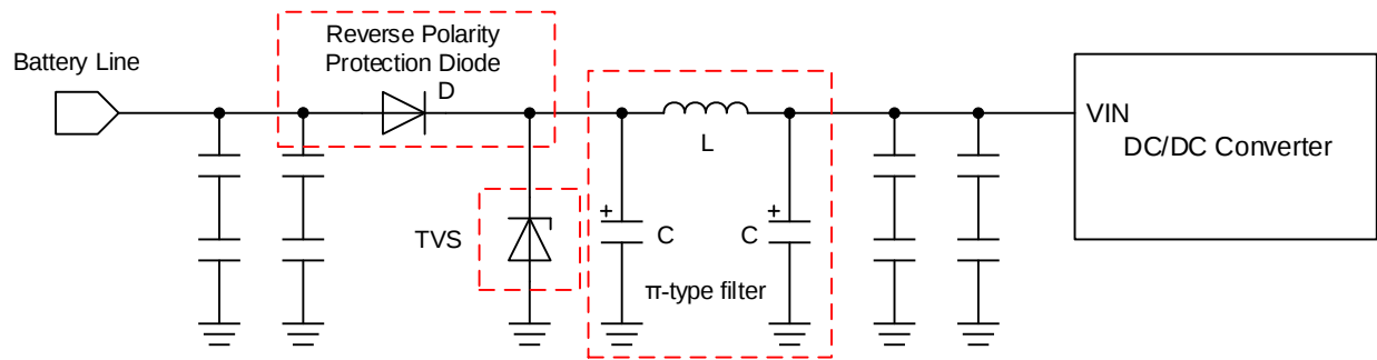
Figure 93. Automotive Power Supply Line Circuit
