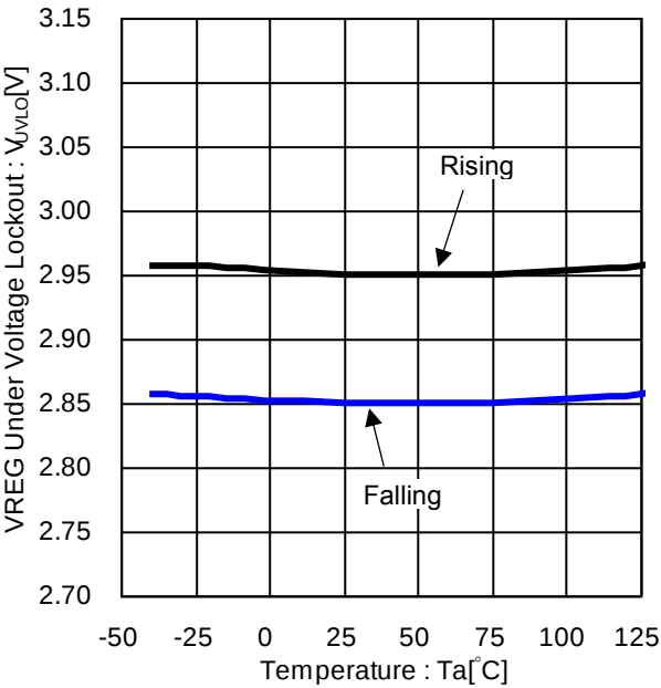
Figure 8. VREG Under Voltage Lockout vs Temperature
