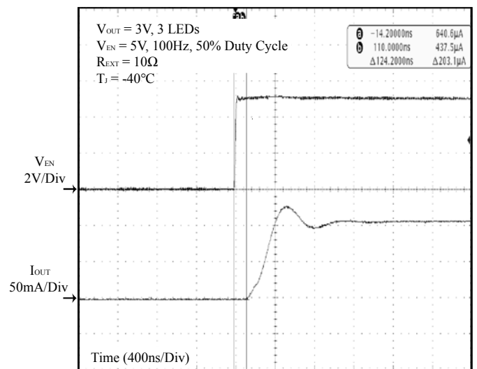
Figure 32 V_{EN} vs. I_{OUT} Delay and Rising Edge
