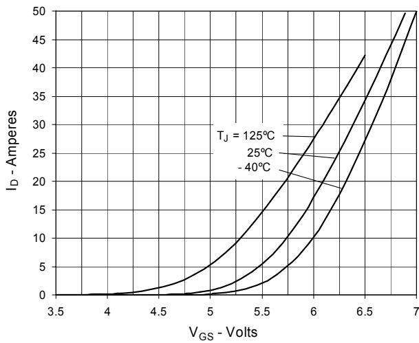
Fig. 7. Input Admittance
