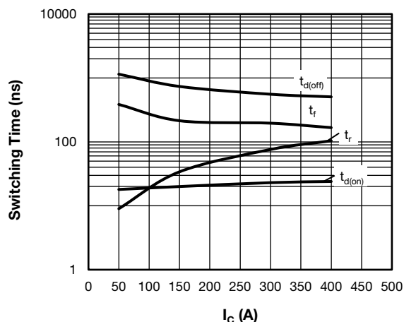
Fig. 8 - Typical Q1 to Q2 IGBT Switching Time vs. I_C (with D1 to D2 Antiparallel Diode)
