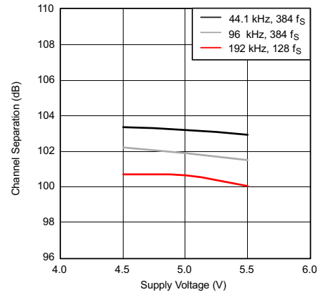
Figure 15. Channel Separation vs Supply Voltage
