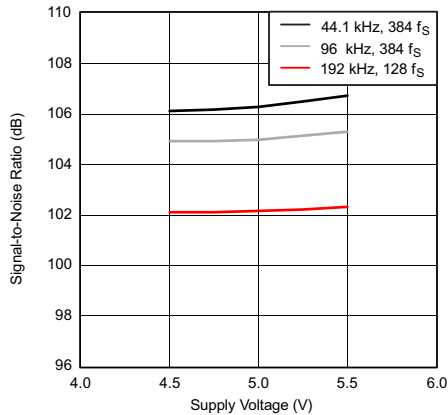
Figure 14. Signal-to-Noise Ratio vs Supply Voltage
