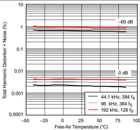
Figure 16. Total Harmonic Distortion + Noise vs Free-Air Temperature
