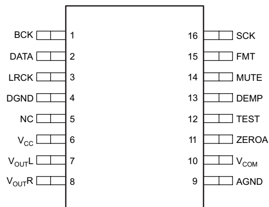
Pin Functions—PCM1754-Q1
