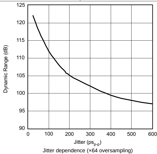
Figure 37. Dynamic Range vs Jitter
