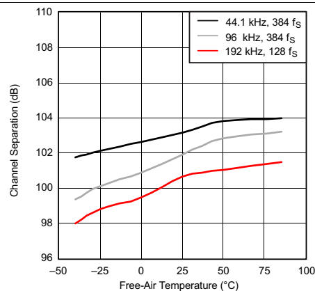
Figure 19. Channel Separation vs Free-Air Temperature
