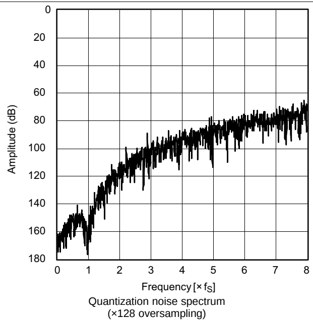
Figure 36. Amplitude vs Frequency
