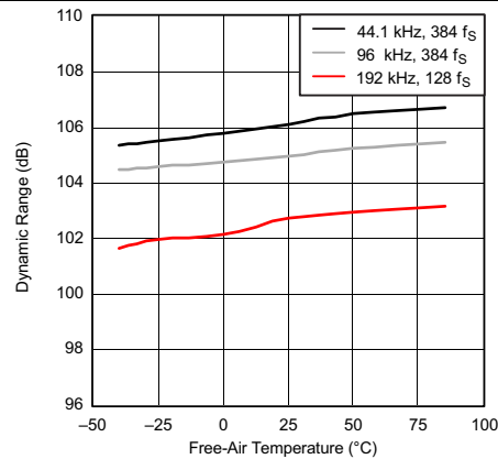
Figure 17. Dynamic Range vs Free-Air Temperature
