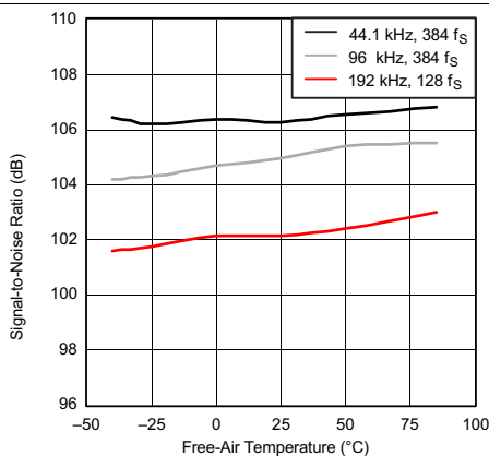
Figure 18. Signal-to-Noise Ratio vs Free-Air Temperature
