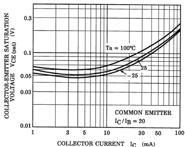
Fig. 10.23 RN1905 V_{CE(sat)}-I_C
