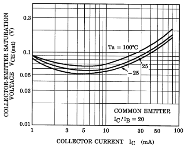
Fig. 10.21 RN1903 V_{CE(sat)}-I_C
