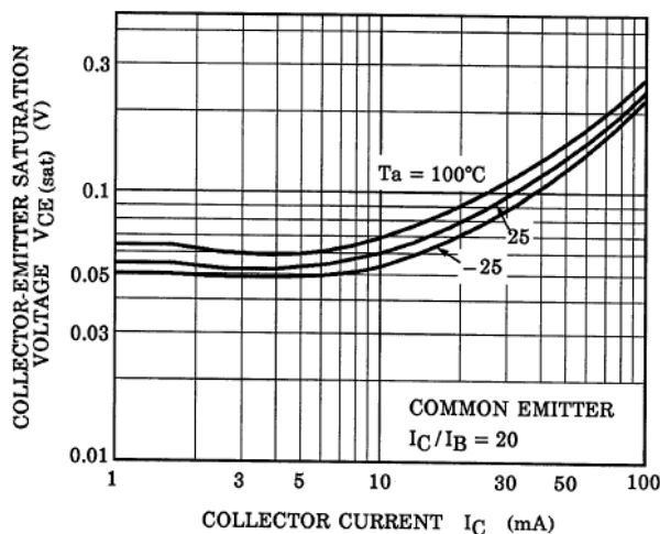
Fig. 10.24 RN1906 V_{CE(sat)}-I_C
