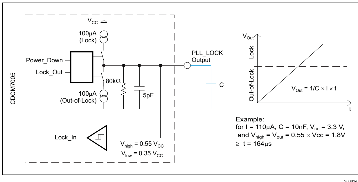
Figure 19. Analog Lock-Detect
