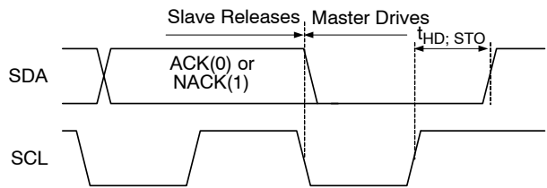
Figure 21. Stop Bit
