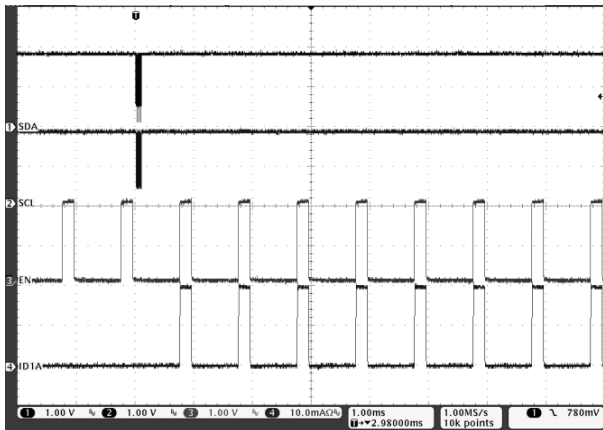
Figure 17. PWM and Linear (Via I 2 C) Dimming, V_{IN} = 3.6\text{ V} , I_{LEDx} = 20\text{ mA} , and EN = 1\text{ kHz} with 20% Duty Cycle
