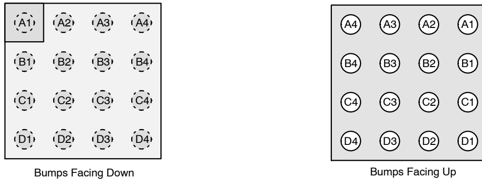
Figure 2. WLCSP-16, 0.4 mm Pitch, 1.61 x 1.61 mm
