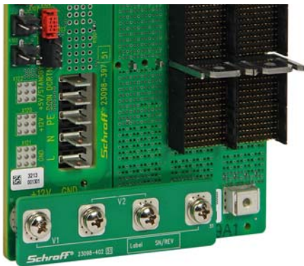
Application: Power backplane (left), CompactPCI Serial backplane (right) and connection via power adapter board (below)
