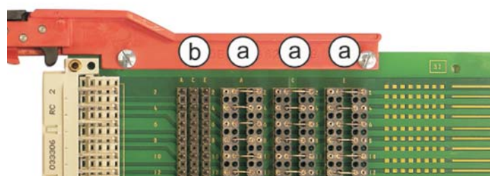
a: Measuring field for current and voltage measurement b: Header for wire wrap
