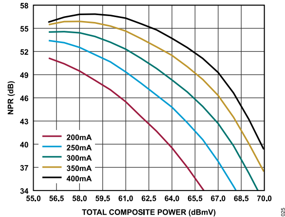
Figure 25. NPR vs. Total Composite Power Over Current, Worst Case Frequency, 10 dB Tilt, V_{DD} = 7.0 V
