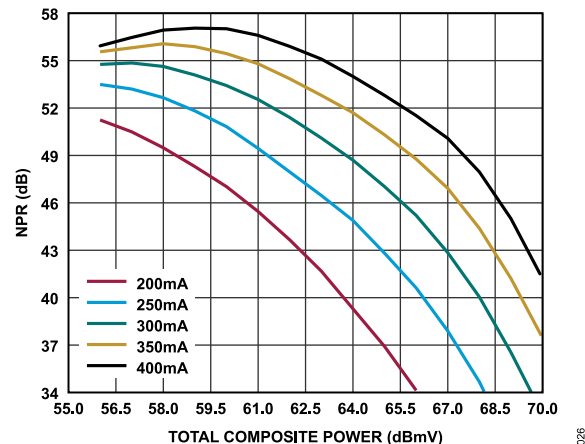
Figure 26. NPR vs. Total Composite Power Over Current, Worst Case Frequency, 10 dB Tilt, V_{DD} = 8.0 V
