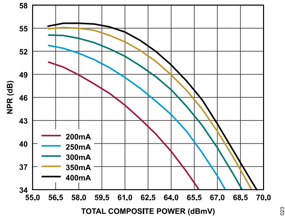
Figure 23. NPR vs. Total Composite Power Over Current, Worst Case Frequency, 10 dB Tilt, V_{DD} = 5.0 V
