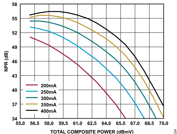
Figure 24. NPR vs. Total Composite Power Over Current, Worst Case Frequency, 10 dB Tilt, V_{DD} = 6.0 V
