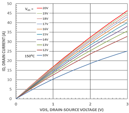
Figure 4. MOSFET Typical Output Characteristics
