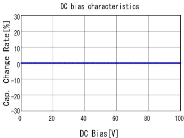
■ GQM1555C2A470JB01 C-DC bias capchange, 25.0degC, AC1V
