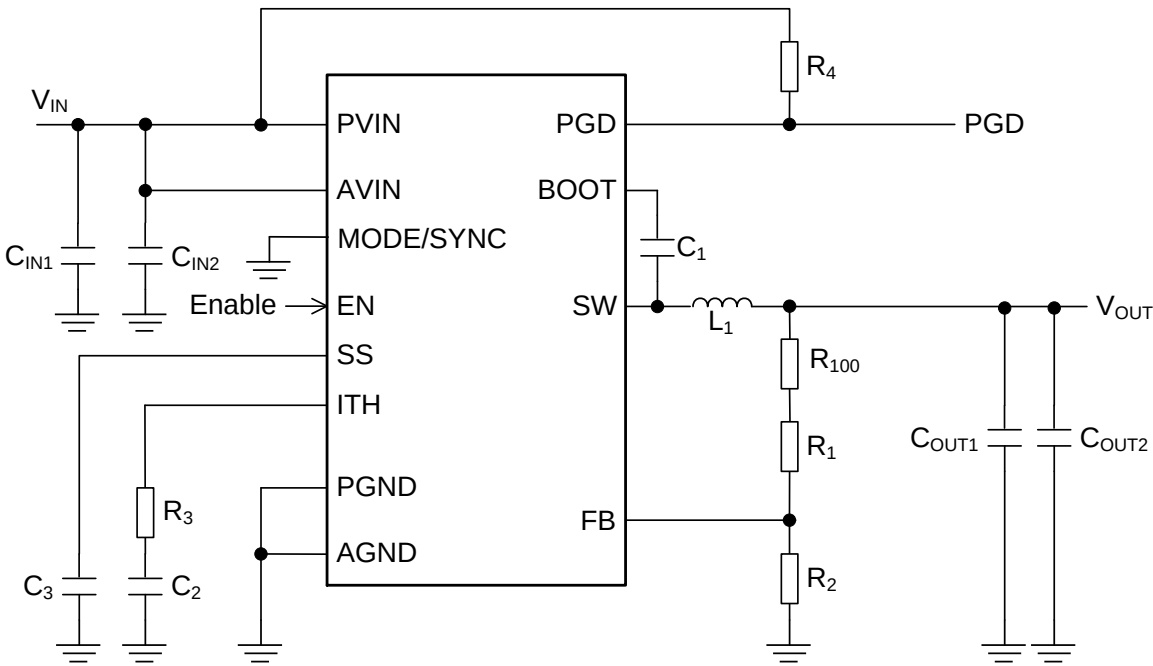
Figure 34. Typical Application
