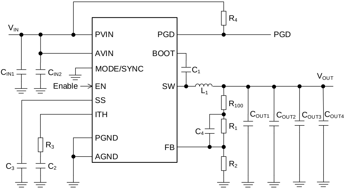
Figure 46. Reference Circuit 2
