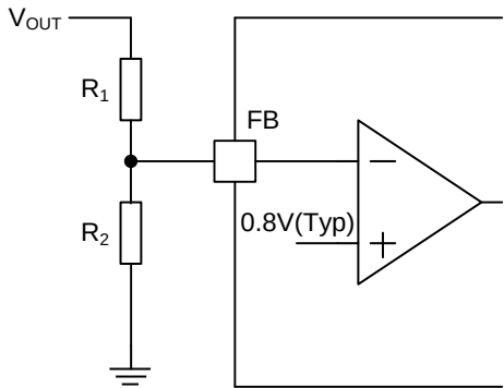
Figure 35. Feedback Resistor Circuit
