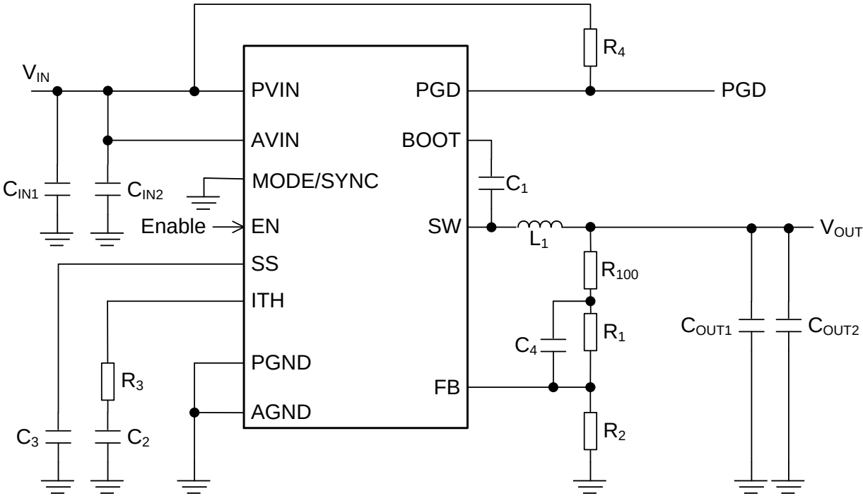
Figure 61. Reference Circuit 5
