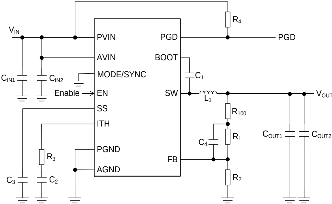
Figure 41. Reference Circuit 1
