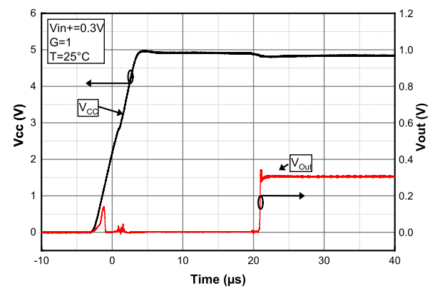
Figure 44. Turn-on time at V_{CC} = 5\text{ V}
