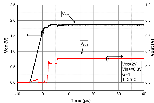
Figure 45. Turn-on time at V_{CC} = 2\text{ V}
