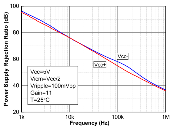
Figure 43. PSRR vs. frequency at V_{CC} = 5\text{ V}
