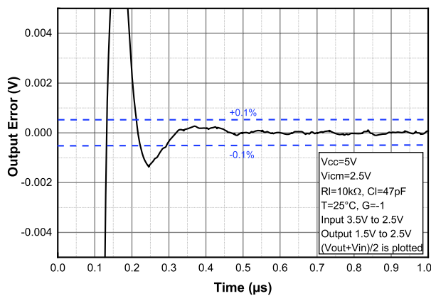
Figure 35. Settling time output low to high at V_{CC} = 5\text{ V}
