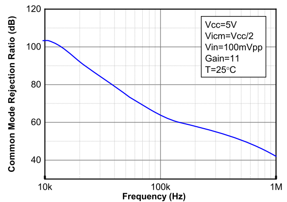
Figure 42. CMRR vs. frequency at V_{CC} = 5\text{ V}
