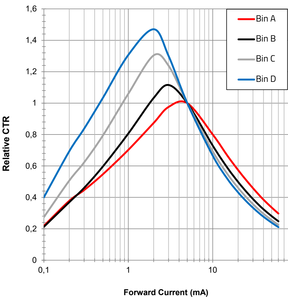
Relative CTR vs. Forward Current ( at V_{CE}=0,4\text{ V} )
