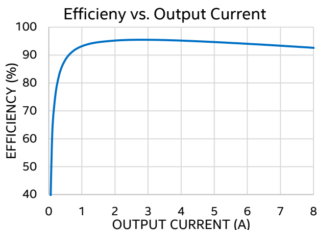
Figure 2: Efficiency at V_{IN} = 5V , V_{OUT} = 3.3V
