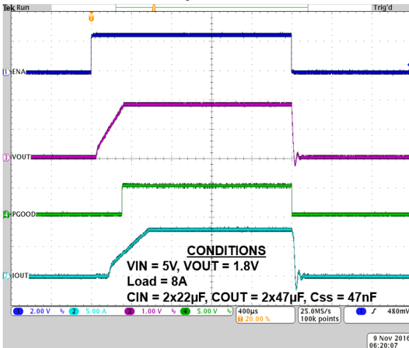
Startup Waveform
