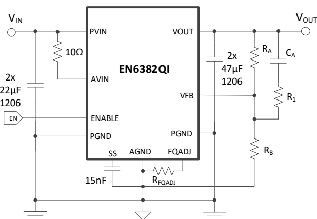
Figure 1: Simplified Applications Circuit
